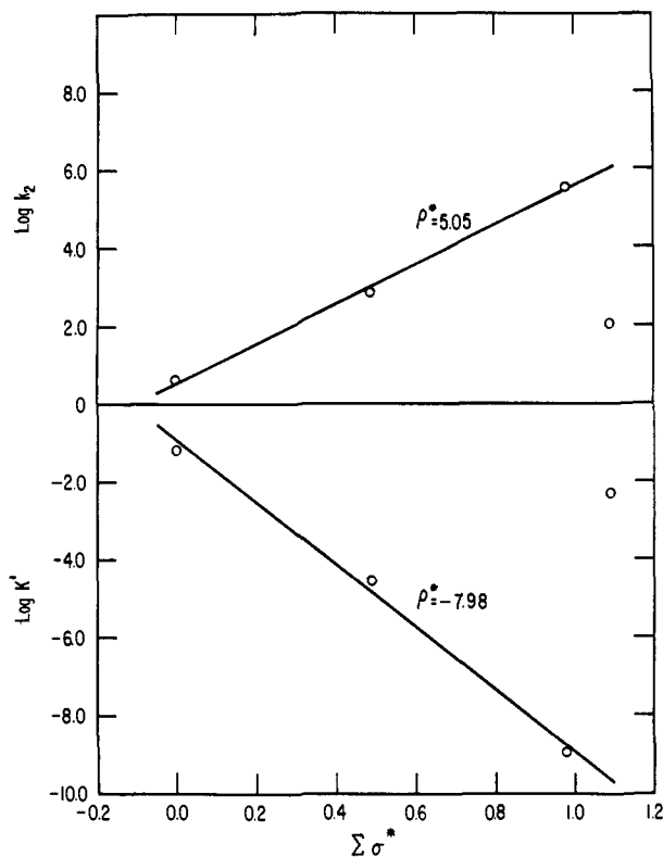
Figure 3. (Upper plot) \text{Log } k_2 vs. \Sigma\sigma^* . (Lower plot) \text{Log } K' vs. \Sigma\sigma^* . \Sigma\sigma^* formaldehyde = 0.98, \Sigma\sigma^* acetaldehyde = 0.49, \Sigma\sigma^* acetone = 0.00, and \Sigma\sigma^* benzaldehyde = 1.09.
