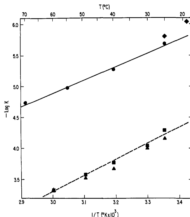
Figure 1. Negative logarithms of equilibrium constants for dissociation of glyconitrile and lactonitrile [RCH(OH)CN ⇌ (RCHO) aq + HCN] vs. 1/T: (●) glyconitrile pK from measured equilibrium between glyconitrile and lactonitrile; (◆) glyconitrile pK from dissociation measurements; (■) lactonitrile pK (Yates and Heider data recalculated with new pK of HCN); (▲) original Yates and Heider data. The solid line is a least-squares fit of the glyconitrile data with the dissociation measurements omitted. The dashed line is a least-squares fit of the recalculated lactonitrile data.
